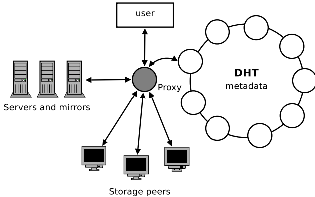
Figure 1. apt-p2p's architecture
